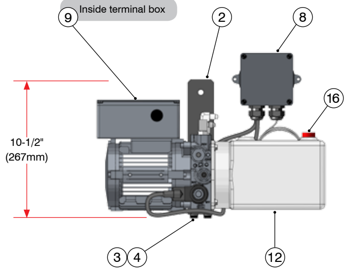
Front View – Wall Mount
