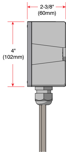
Junction Box - Side View
