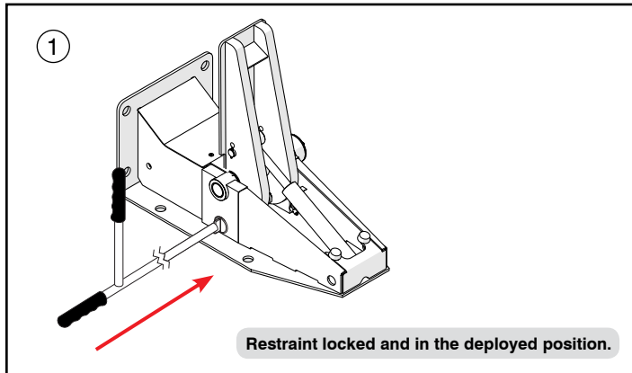
Insert un-locking bar (Part# 54-001682) into slot with pressure for leverage.
